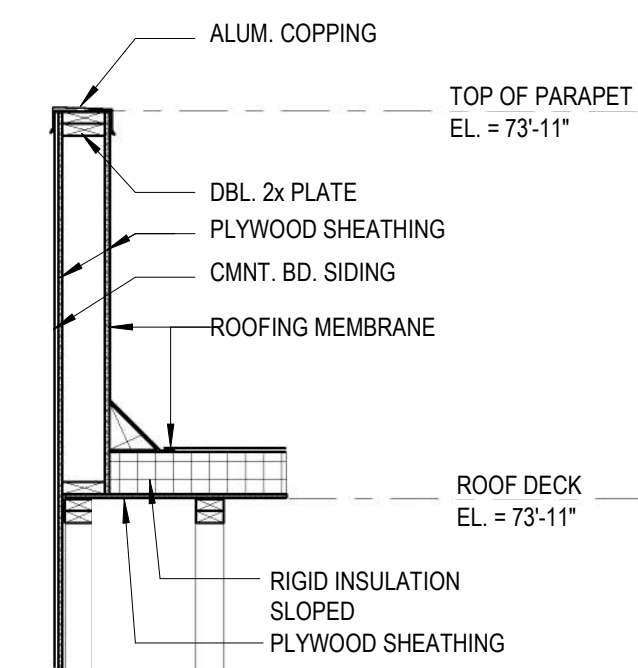
2 PARAPET DETAIL (TYP.) 1/2" = 1'-0"
